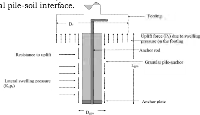
Fig 1. Concept and the forces acting on a GPA
