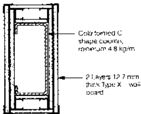
Fig.9 Board protection for columns beams
