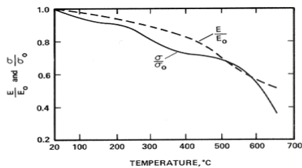
Figure 7: Effect of temperature on modulus of elasticity (E) and yield stress (σ) for steel
