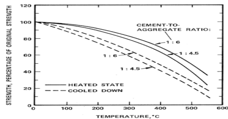
Figure 8: Effect of temperature on compressive strength of concrete
