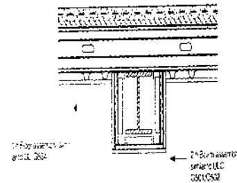
Fig.10 Gypsum board protection for beams
